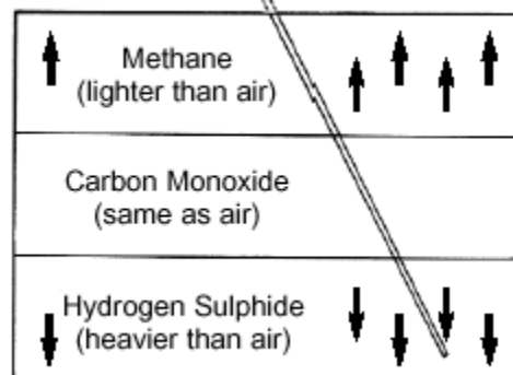
Figure 7. Monitoring of the atmosphere can be conducted from outside the confined space and during occupancy of the space with a continuous monitoring device, which usually has audible and/or visual alarms.
