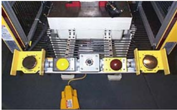
A two-handed control option may be suitable to ensure that a machine can not operate until both hands of the operator are clear of the hazard area.
